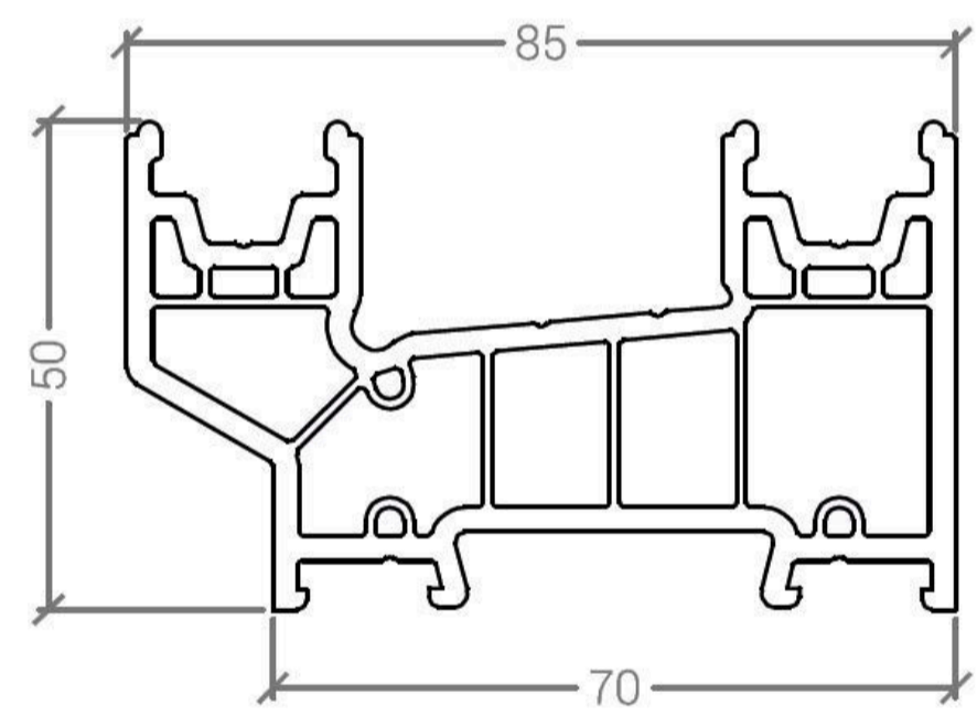
Outer Frame
