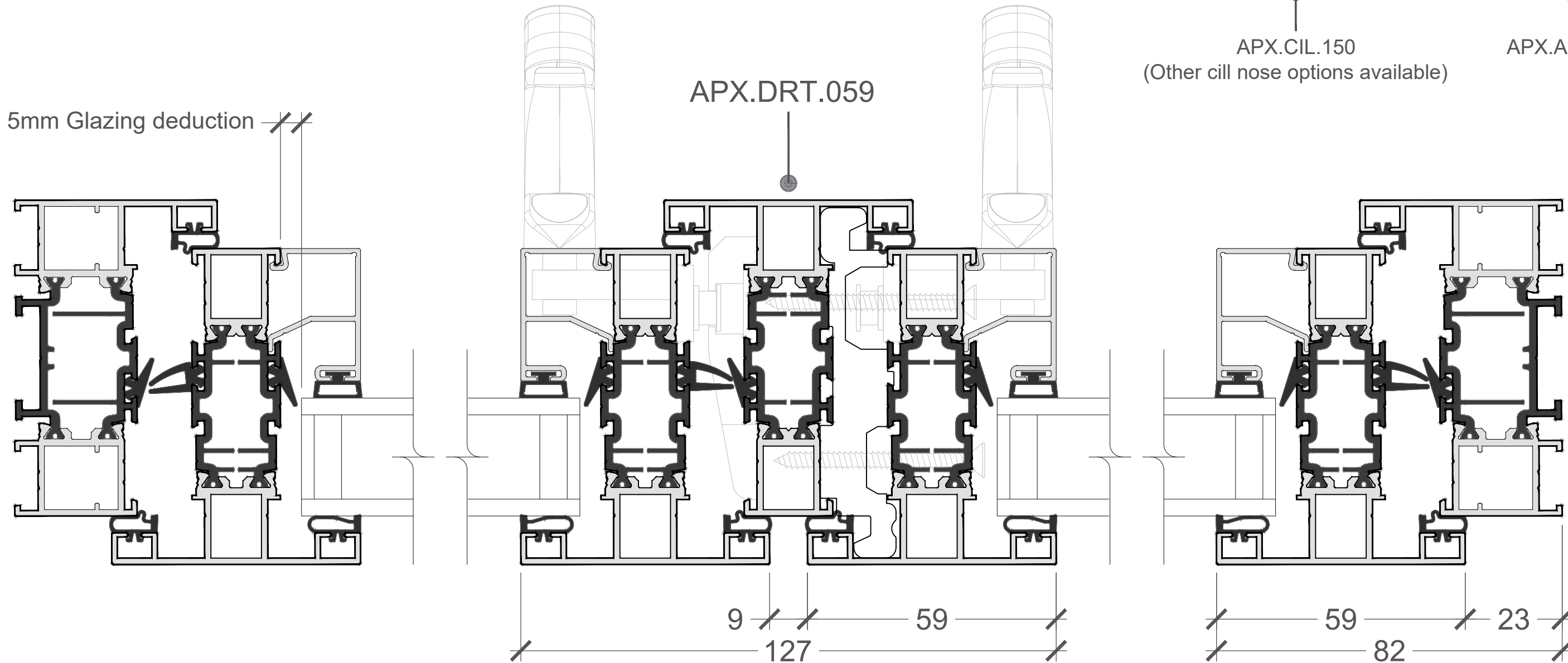
Section "c-c"
