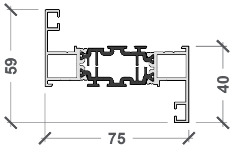
APW.DRZ.059 59MM DOUBLE REBATE Z
