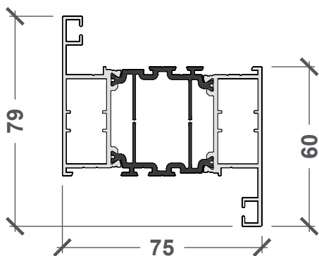
APW.DRZ.079 79MM DOUBLE REBATE Z
