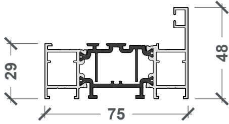
APX.SRS.048 48MM SINGLE REBATE STANDARD
