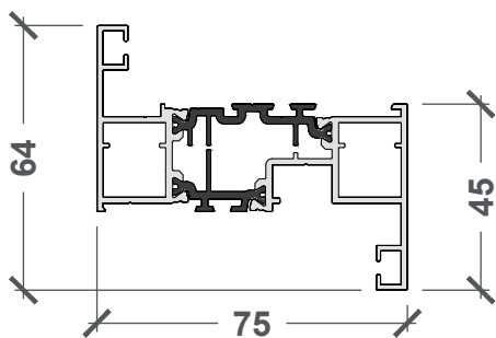
APW.TTS.064 64MM TILT TURN SASH
