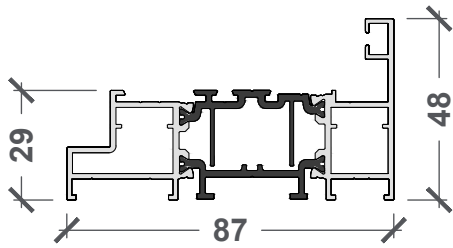
APW.SRF.048 48MM SINGLE REBATE FLUSH
