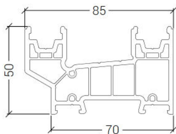
Outer Frame
