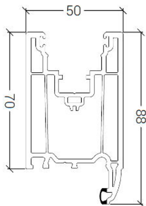
Sash
