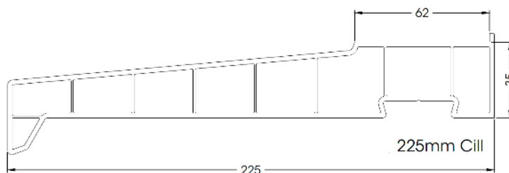
180mm Cill
