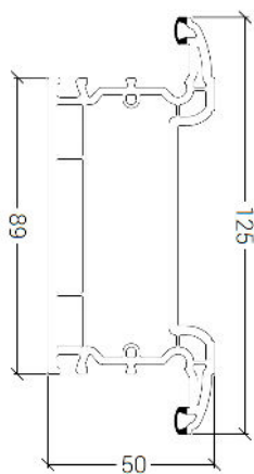
Midrail
