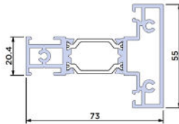
Transom for Sash BF73.0301
