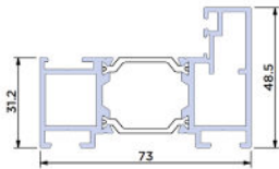
Super Slim Sash (48.5mm) BF73.0203
