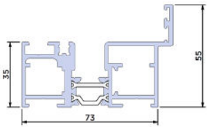
Standard Outer Frame (55mm) BF73.0101
