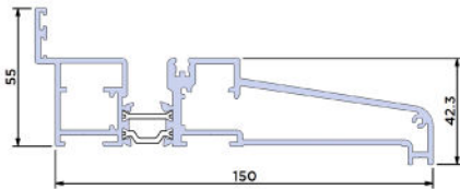
Integrated Outer Frame and 150mm Cill BF73.0111
