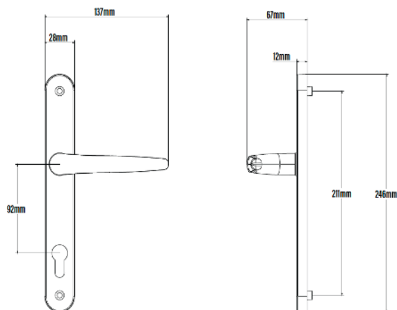
Lever/Lever Handle
