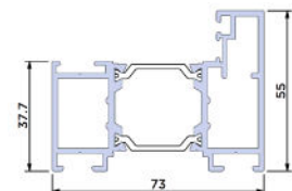
Slim Sash (55mm) BF73.0201
