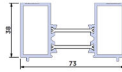
38mm Add-on BF73.0503
