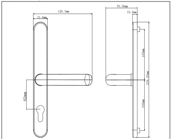
OFFSET LEVER/LEVER EXTERNAL HANDLE
