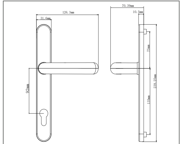
INLINE LEVER/LEVER EXTERNAL HANDLE
